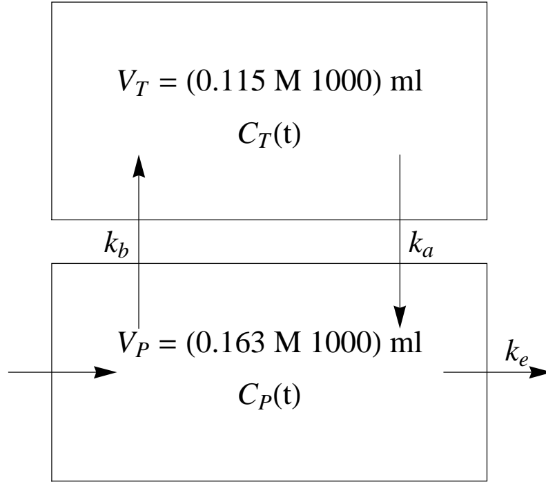
Figure 1. Two compartment model for LSD flow between plasma and tissue compartments in the human body where the volume (in milliliters) of the plasma ( V_P ) is 16.3% of the volume or mass ( M ) of the body and the volume of the tissue ( V_T ) portion of the body is 11.5% of the volume or mass of the body.
